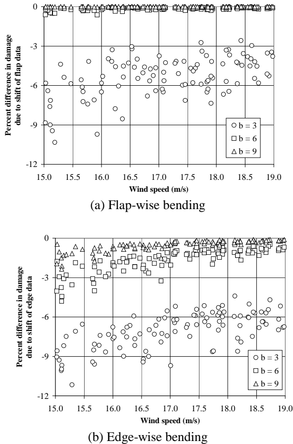
Figure 5 Effect on damage estimation of shift in blade bending moment range data.
