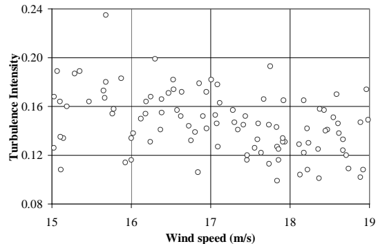
Figure 1 Wind speed and turbulence intensity values for the 101 10-minute data samples.
