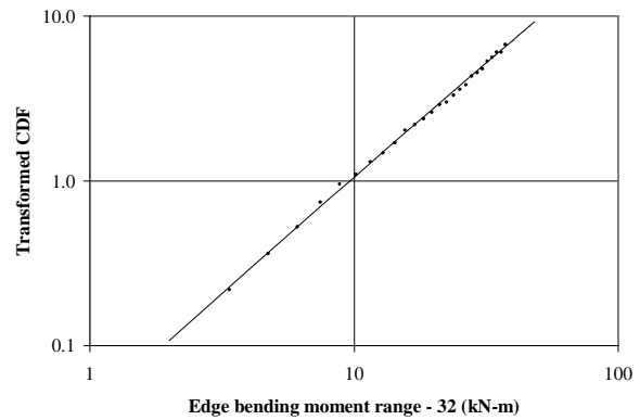
(b) Weibull scale plot (truncation at 32.0 kN-m)
