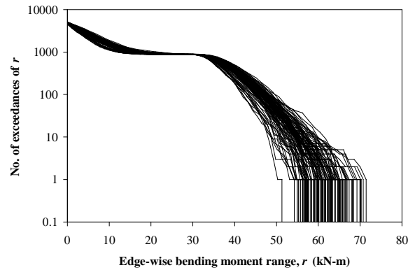
Figure 2d Cumulative counts of flap-wise bending moment ranges for 101 10-minute data sets.
