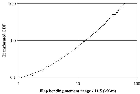
(b) Weibull scale plot (truncation at 11.5 kN-m).
