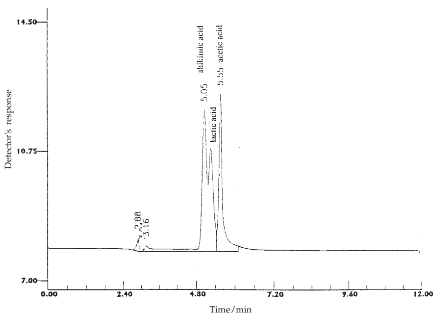
Fig. 3. Separation of shikimic, lactic and acetic acids on RP-HPLC column under the same conditions as in Fig. 2
