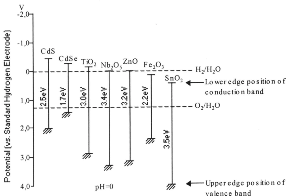
Fig. 3: Band-edge energies of typical semiconductors
