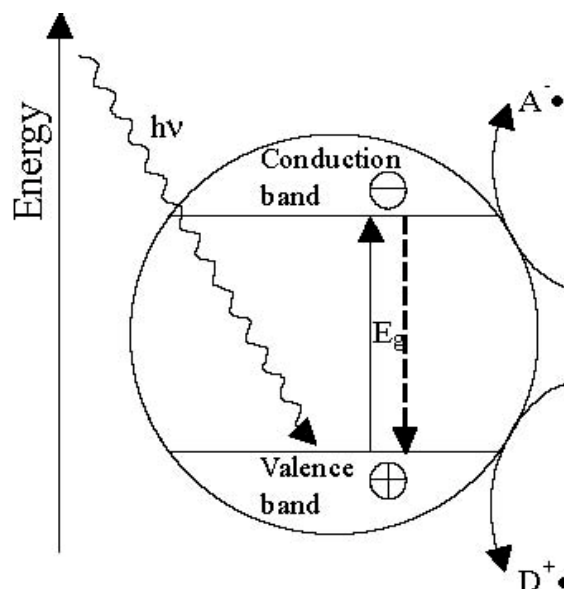
Fig. 2: Operation of a photochemical excited \text{TiO}_2 particle
