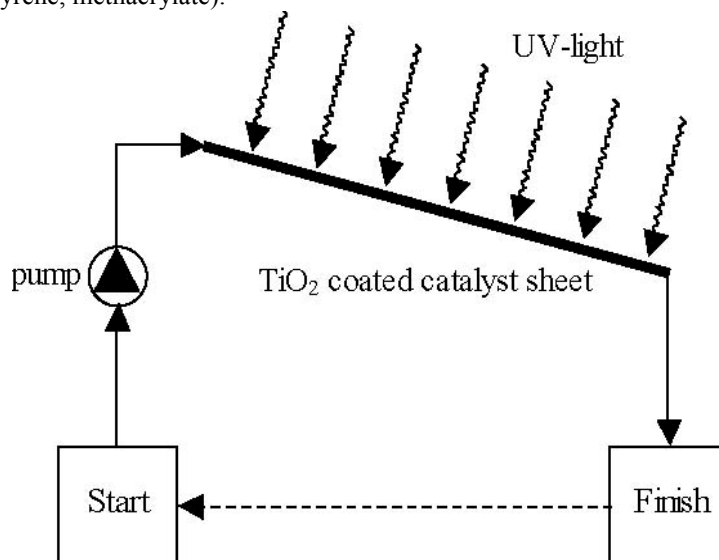
Fig. 5: Thin-film-fixed-bed reactor [5]
